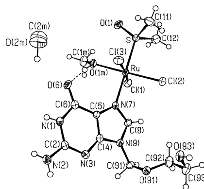
Figure 1. View of the asymmetric unit of 1 ; selected bond lengths (Å): Ru–Cl(1) 2.309(2), Ru–Cl(2) 2.326(2), Ru–Cl(3) 2.362(2), Ru–S 2.270(2), Ru–O(1m) 2.072(6), Ru–N(7) 2.127(5), O(6)–C(6) 1.245(8)
