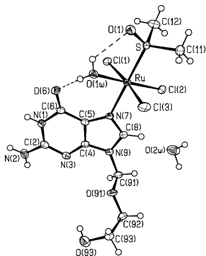
Figure 2. View of the asymmetric unit of 2 ; selected bond lengths (Å): Ru–Cl(1) 2.3686(4), Ru–Cl(2) 2.3187(5), Ru–Cl(3) 2.3210(6), Ru–S 2.2677(5), Ru–O(1w) 2.077(1), Ru–N(7) 2.132(2), O(6)–C(6) 1.247(3)
